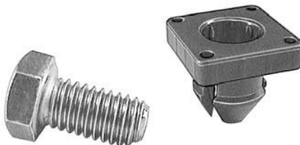
19281 (F5RZ-5421416B) Door Window Glass To Regulator Fastener Assembly 3/8"-16 x 3/4" Grade 8 Cap Screw Contour & Mystique 1995-On
